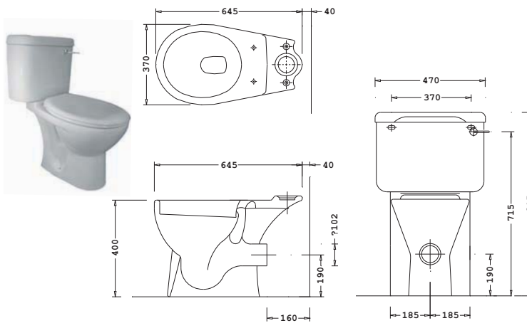
close coupled raised height wc suite (lever flush)
