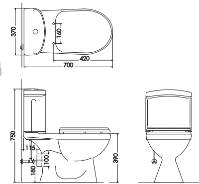
close coupled wc suite (push button)
