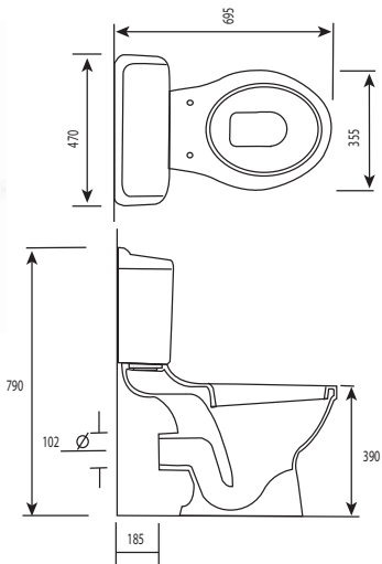
close coupled wc suite lever flush
