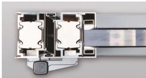
The fire protection core, which is anored in the middle, leaves space free on each side, which can be used for cable routing or for fastening add-on parts.
