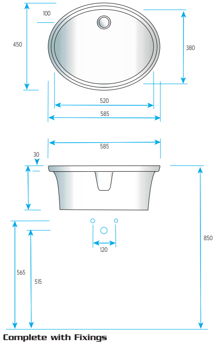
S7004026 - OL25 Under Counter Basin
