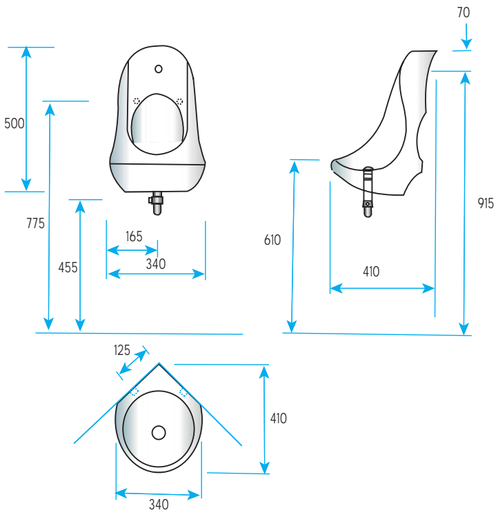
S7004072 - OL95 Corner Urinal Bowl
