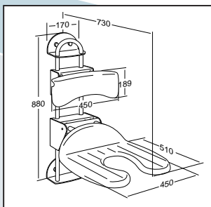
SHOWER CHAIR
