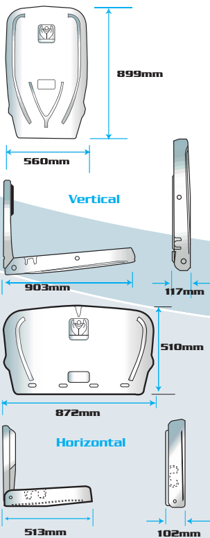
Babyminder Infant Safety Seat
