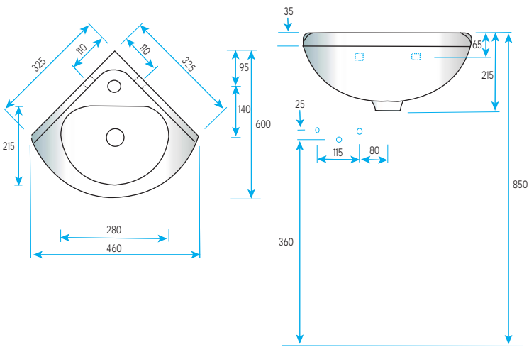
S7004015 - OL26 32cm Corner Basin (Taphole 1) Wall Fixed S7004034 - Hanger Brackets
