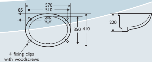
S2084001 - 57cm Oval Plug Bowl No Overflow Complete with Fixing Clips
