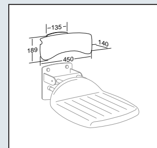
Back Rest
