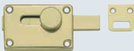
INDICATOR BOLT H8000167 - Internal 60mm x 40mm External 50mm x 50mm
