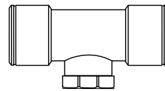
S9920068 - 22 x 22 x 15mm Reducing Tee S9920069 - 22 x 15 x 15mm Reducing Tee S9920070 - 15 x 15 x 22mm Reducing Tee
