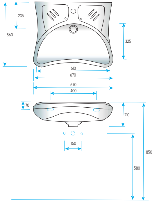
P7004010 - OL20 Shampoo Basin (Taphole 1) (C/W Wall Fixings)
