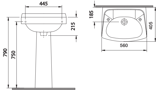
S7006015 - OL60 560x405mm Basin Tapholes 2 (For Towel Rail brackets to wall fix this Basin see page 142)
