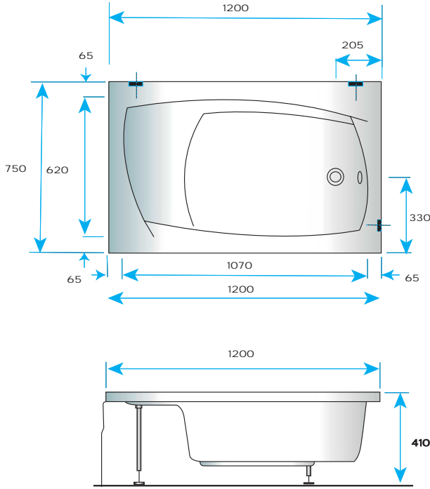
P6808585 - 120 x 75cm
