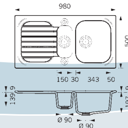
1.5 Bowl Single Drainer (1.5B SD) 1 taphole (reversible) and includes basket strainer waste
