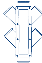
TD17 INSPECTION CHAMBER (TWO BRANCHES EACH SIDE)
