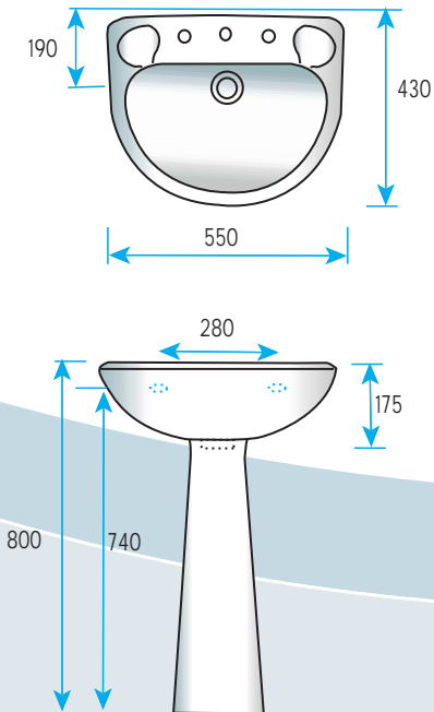
S7006001 - OL50 55cm Basin (Taphole 1) S7006002 - OL51 55cm Basin (Taphole 2) S7006003 - OL52 Pedestal
