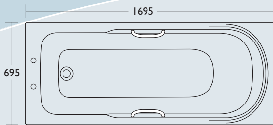
Baronet Bath, height, floor to rim 490-540mm
