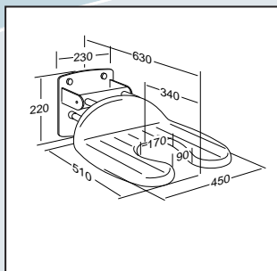
Folding Seat
