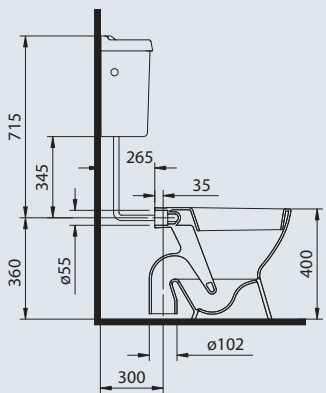
S7006012 - OL58 'S' Trap W.C. Pan
