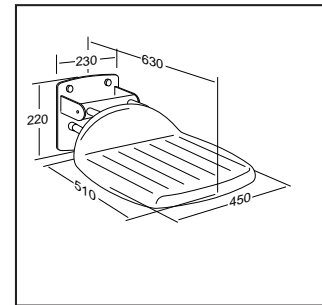
Folding Seat
