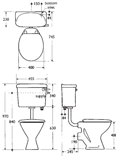
S2000196 - 'S' Trap W.C. Pan
