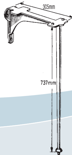
S2063521 - Leg And Bearer Support Twin Pinned Centre Bracket 305mm Stud, Finish Painted Iron
