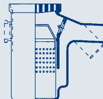
TD554 GARAGE GULLY (300 X 600MM DEEP)
