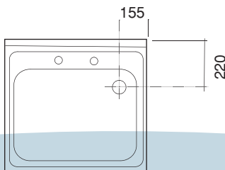
S3025001 - Overall Size: 750 x 650mm
