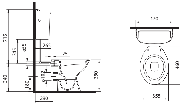
S7006013 - OL59 Low Level Cistern Shell (S.I.S.O) S7006014 - Fitting Pack for above with C.P. Front Lever. (Internal/External Overflow)
