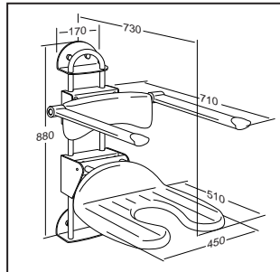
SHOWER CHAIR
