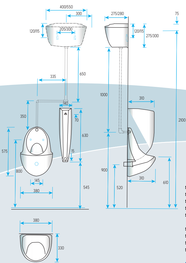
S7004044 - OL38 Concealed Trap Urinal Bowl S7004028 - OL23 Urinal Division S2199031 - 4.5 Ltr Concealed Plastic Auto Cistern S2199032 - 9.0 Ltr Concealed Plastic Auto Cistern S2199033 - 13.5 Ltr Concealed Plastic Auto Cistern S2195501 - Concealed Pipes & Spreaders (1 person) S2195511 - Concealed Pipes & Spreaders (2 person) S2195521 - Concealed Pipes & Spreaders (3 person) S2195531 - Concealed Pipes & Spreaders (4 person)
