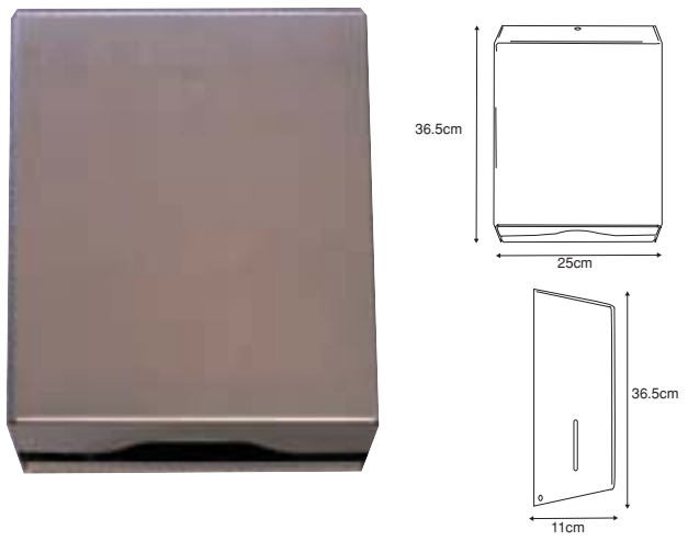
S2942011 - Brushed S/Steel Hand Towel Dispenser. Locking Cover S2942012 - Interleaved Paper Towels
