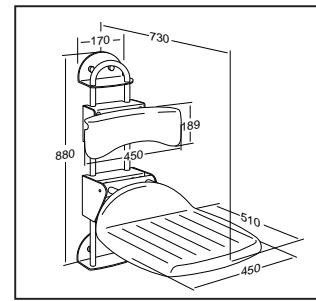
SHOWER CHAIR
