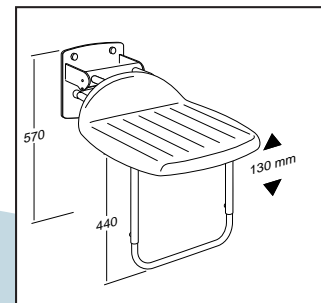
Folding Seat
