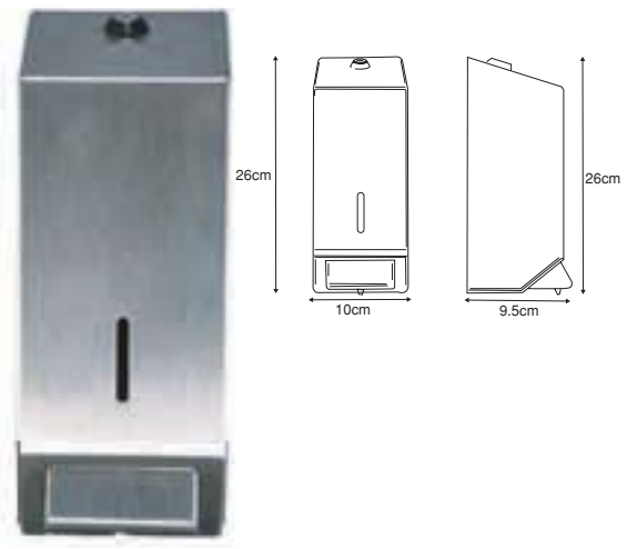
S2942010 - Brushed S/Steel 1 Ltr Refillable Soap Dispenser. Locking Cover
