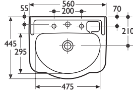
S7001058 - 56cm Semi Countertop Basin TH1 White
