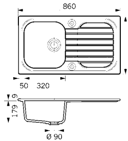
Single bowl Single drainer (SB SD) 1 taphole (reversible) and includes basket strainer waste
