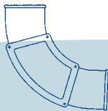
TD09 MEDIUM RADIUS BEND SIDE ACCESS
