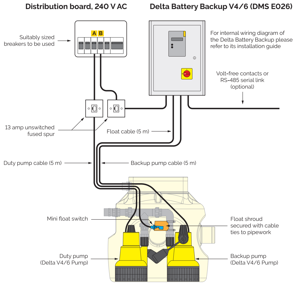
Delta Dual V4/6 packaged pumping station (DMS 217/079)
