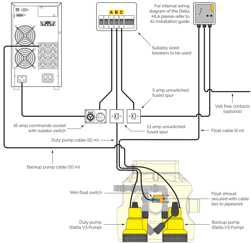
Delta Dual V3 packaged pumping station (DMS 164)
