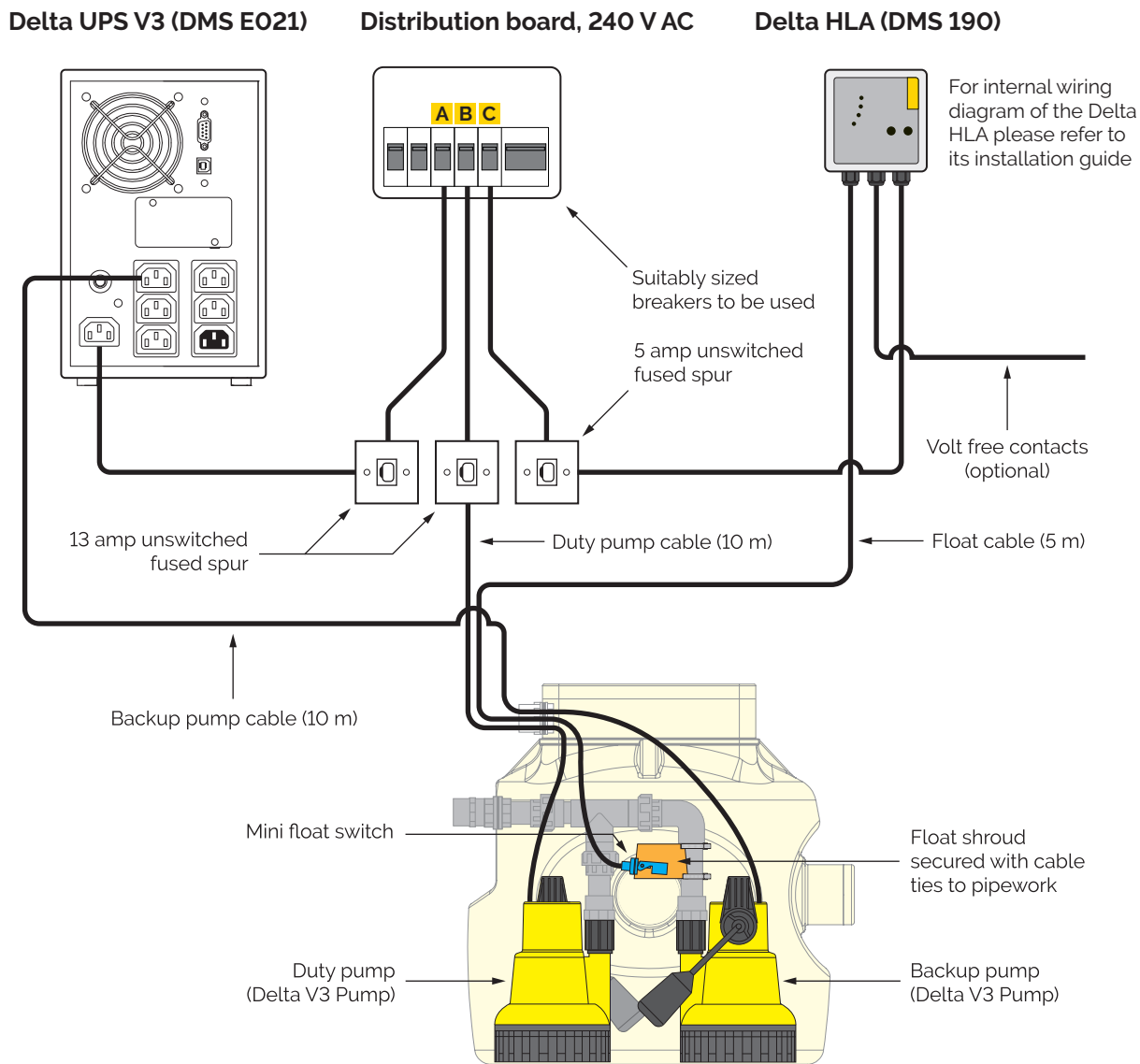
Delta Dual V3 packaged pumping station (DMS 164)
