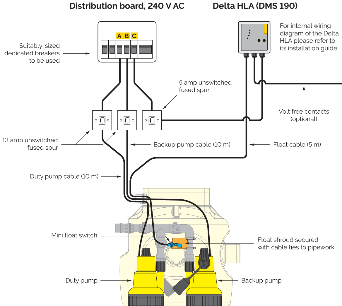
Delta Dual V3 packaged pumping station (DMS 164)
