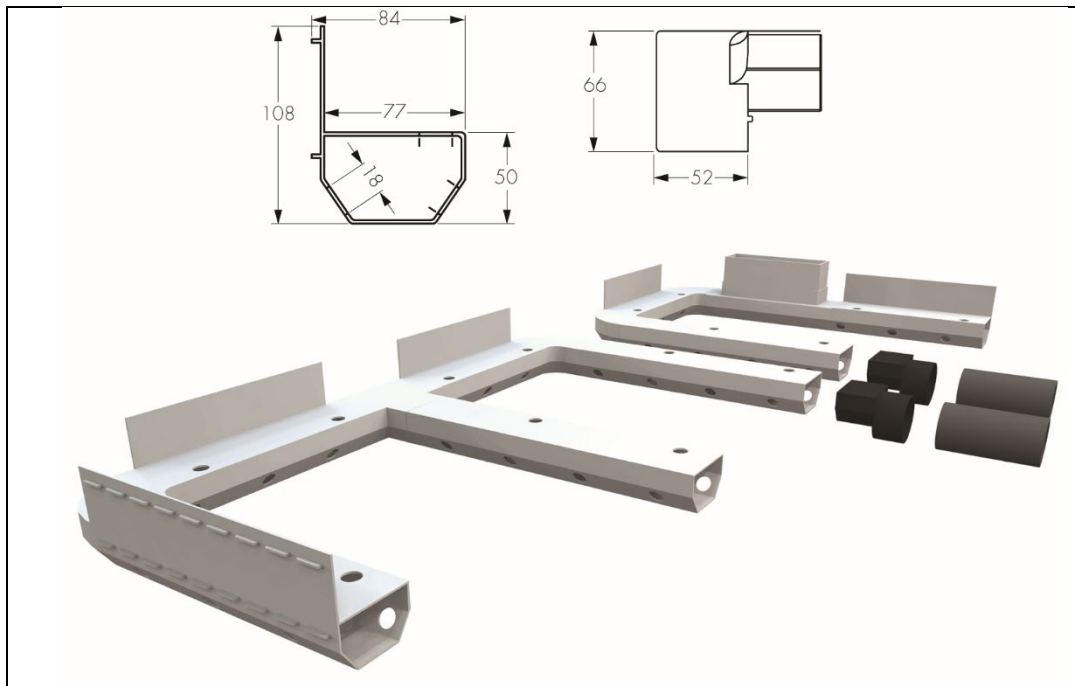
Figure 1 Newton Basedrain (all dimensions in mm)
