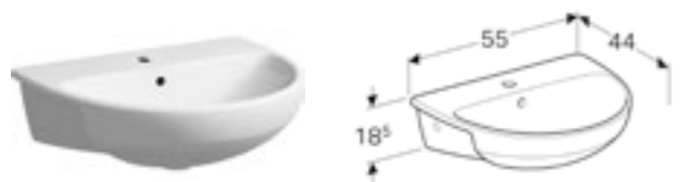
Geberit Selnova 55cm semi-recessed washbasin W 55 / D 44 / H 18.5cm Visible overflow.
