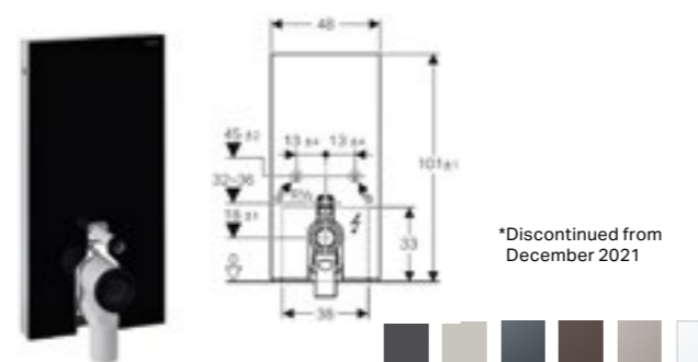
Geberit Monolith Plus W 48.2 / D 10.6 / H 101cm Floor standing toilet, height 101cm. Art. no. Product Description RRP ex VAT 131.202.TG.5* Black glass / aluminum € 2,287.05 131.202.SQ.5* Umber glass / aluminum € 2,287.05 131.202.SJ.5* Sand glass / aluminum € 2,287.05 131.202.SI.5 White glass / aluminum € 2,287.05 131.202.JK.5 Lava glass / black chrome aluminium € 2,287.05 131.202.JL.5 Sand grey glass / aluminium € 2,287.05 131.202.JV.5 Stoneware concrete look / aluminium € 2,436.86 131.202.00.5 Stoneware slate look / black chrome aluminium € 2,436.86 131.202.SJ.6 Black glass / black chrome aluminium € 2,287.05
