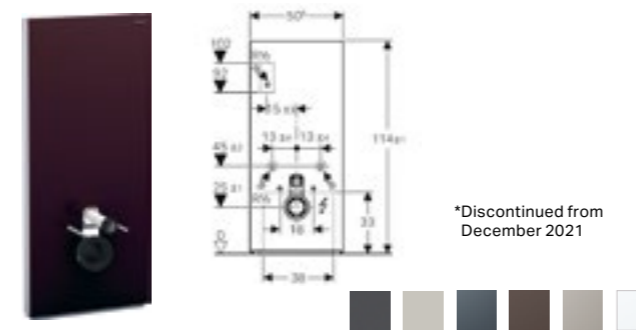
Geberit Monolith Plus W 50.5 / D 10.6 / H 114cm Wall-hung toilet, height 114cm. Art. no. Product Description RRP ex VAT 131.231.SJ.5* Black glass / aluminum € 2,433.04 131.231.SQ.5* Umber glass / aluminum € 2,433.04 131.231.TG.5* Sand glass / aluminum € 2,433.04 131.231.SI.5 White glass / aluminum € 2,433.04 131.231.JK.5 Lava glass / black chrome aluminium € 2,433.04 131.231.JL.5 Sand grey glass / aluminium € 2,433.04 131.231.JV.5 Stoneware concrete look / aluminium € 2,583.15 131.231.00.5 Stoneware slate look / black chrome aluminium € 2,583.15 131.231.SJ.6 Black glass / black chrome aluminium € 2,433.04
